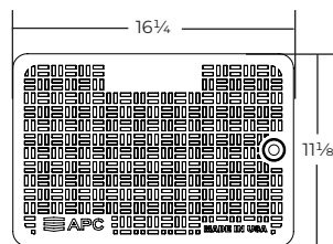
T-COVER THICKNESS: 2"
