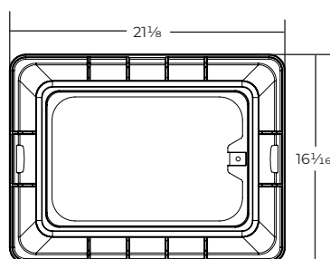
T-COVER THICKNESS: 2"
