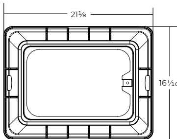
T-COVER THICKNESS: 2"
