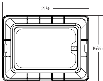
T-COVER THICKNESS: 2"
